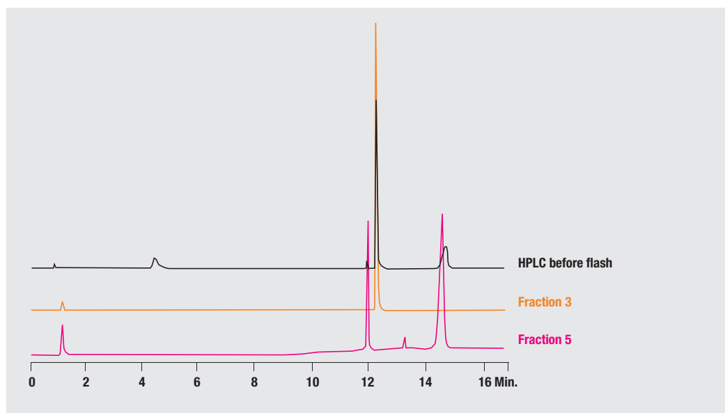
HPLC Chromatograms of giant knotweed fractions collected by Reveleris ® flash chromatography.
