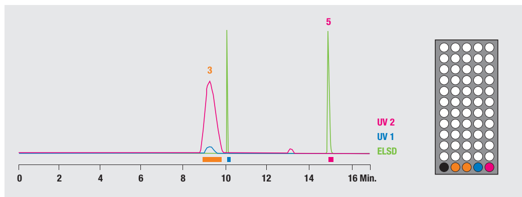
Separation of chromophoric and non-chromophoric compounds in giant knotweed flash chromatography.
